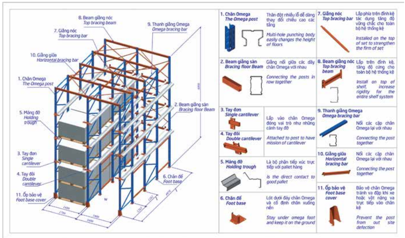
Cấu tạo kệ Drive-in/ Detail of Drive-in rack
